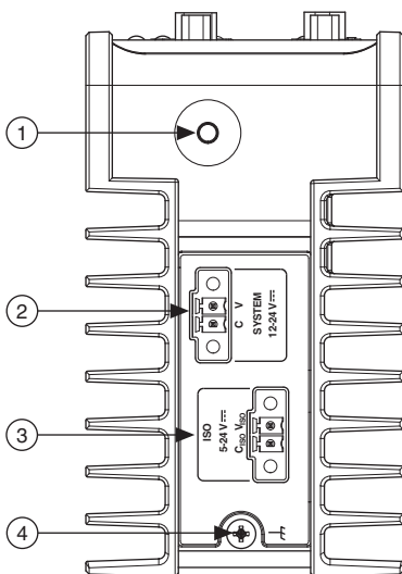
Figure 1. NI CVS-1459RT Power Connectors and Reset Button
