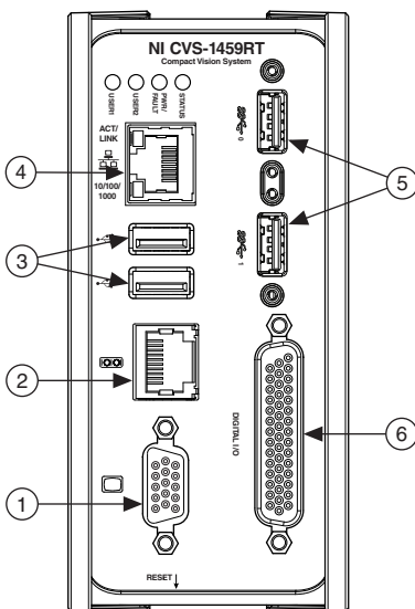
Figure 2. NI CVS-1459RT Front Panel Connectors
