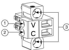
Figure 3. Power Screw Terminal Connector Plug
